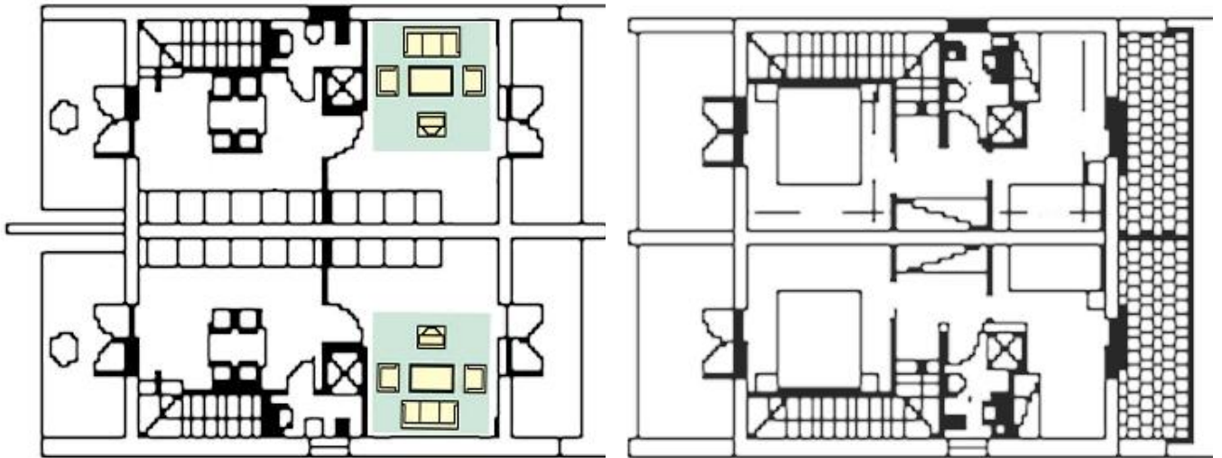
Layouts for the townhouses, Iasca Dreams and Iasca Calabretta
